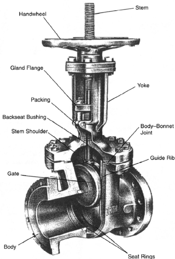
รูปที่ 3-1 Flanged end, Bolted-Bonnet, Outside-Screw-and-Yoke, Flex-Wedge, Gate Valve
