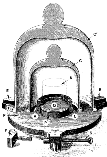
Fig. 22.8. Sectional view of an original container for a kilogram prototype: K Pt-Ir kilogram prototype; Q Quartz plate as flat surface for the prototype; P, P' Base plate (P) with brass cylinder (P'); A Brass crown (L) with silver ring (A) (inner diameter 42 mm) for protection against possible side movements of the prototype; C, C' Glass bell-jars secured against side movement by a ridge on the base plate (P); E, F Fixtures securing the outer glass bell-jar (C). Fixture E is attached, Fixture F is removable; S Safety device for the removable fixture (F); The international prototype is additionally protected by a third glass bell-jar which lies on a polished glass plate (Fig. 22.6).
