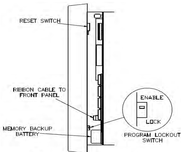
Figure 1. The Program Inhibit Switch
