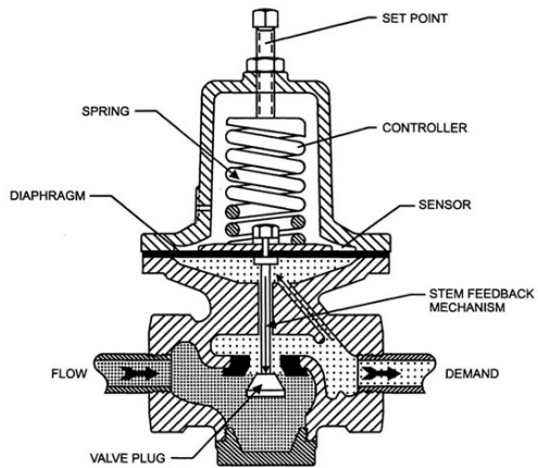
Regulator
