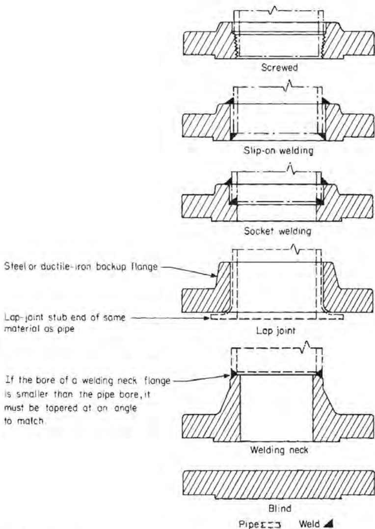
FIG. 10-133 Types of carbon and alloy steel flanges.
