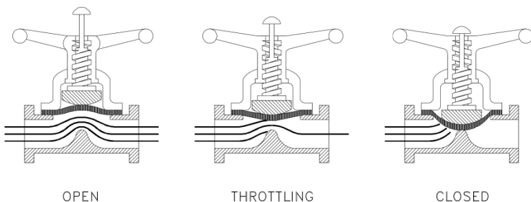
ข. Weir Diaphragm Valve
