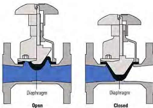
ก. Straight-through Diaphragm Valve
