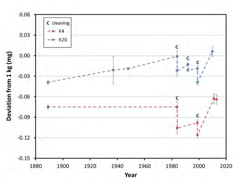
Fig. 1. History of the calibration of the U.S. National Prototype K20 and check standard K4 at the BIPM. The uncertainty bars ( k=1 ) for each number are the uncertainties reported by the BIPM on the calibration certificates. No uncertainty was reported on the 1948 calibration of K20.
