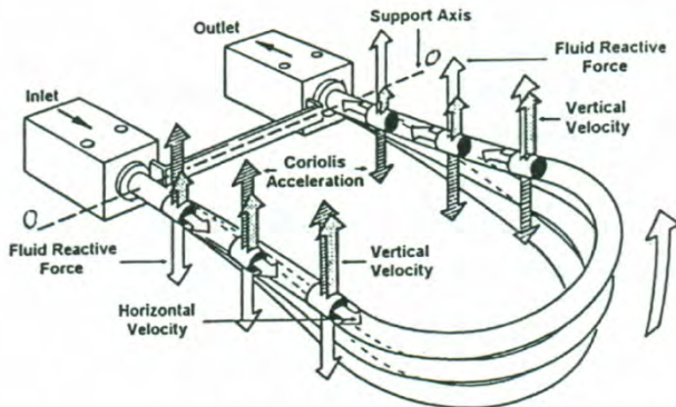
Flow Tube Response to Coriolis Acceleration
