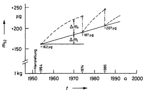
Fig.22.9. Changes in mass of the kilogram prototype No.52. \Delta m_i irreversible, longstanding increase in mass. \Delta m_r reversible increase in mass due to surface layers that are removed by cleaning.
