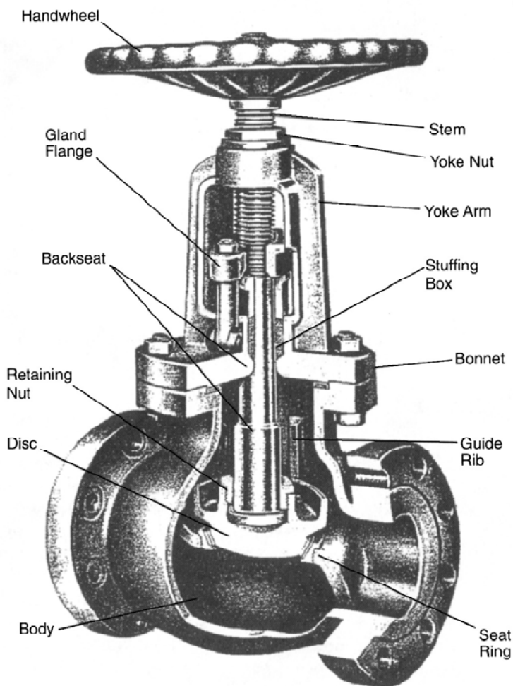
รูปที่ 3-17 Flanged end, Bolted-Bonnet, Outside-Screw-and-Yoke, Spherical Disc, Globe Valve
