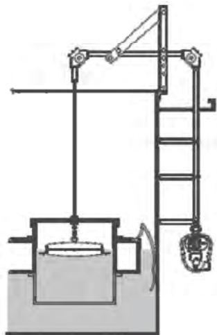
Floating Roof Tank and Float Well
