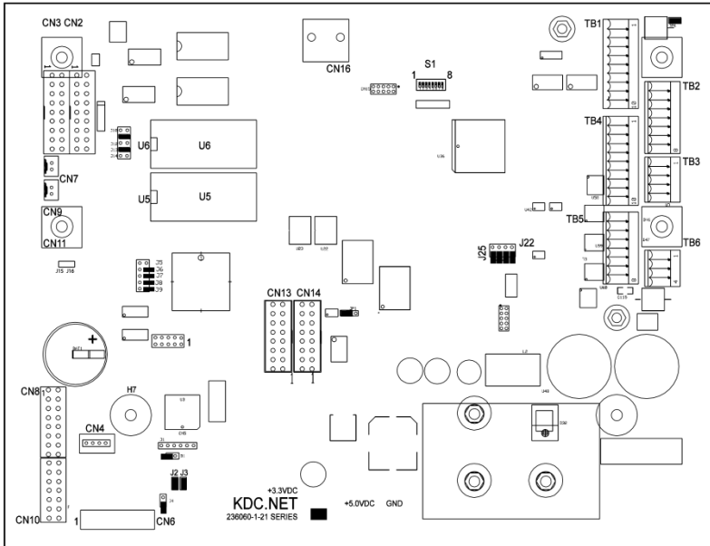
Figure 5. KDC Layout
