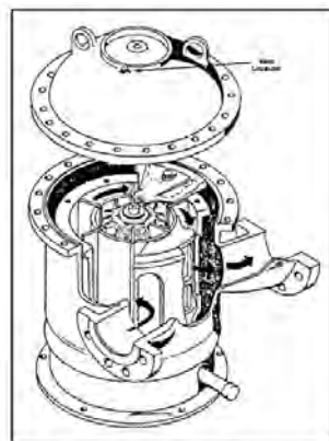
Figure 2 – High Capacity Double Case Meter
