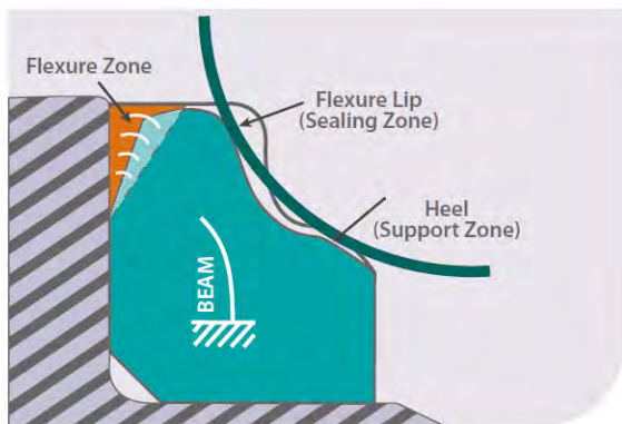
FIGURE 1- Flexible Lip Seat Design: The Jamesbury Flexible Lip Seat is a unique seat lip and heel design. Deflection of the flexible lip allows the seat to store energy. The flexible lip contacts the ball in the sealing zone, while the heel supports the ball as a bearing surface. The valve body design includes a specific flexure zone that allows the seat to flex but prevents excessive movement that would cause permanent deformation.
