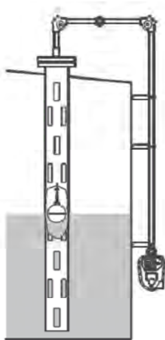
Cone roof tank with Stilling Well
