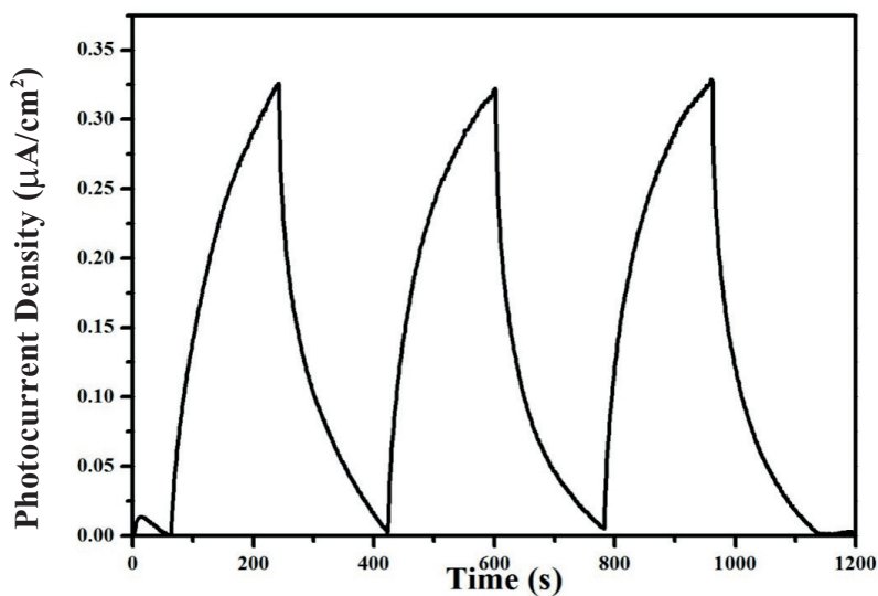
Figure 6 Time-dependent photocurrent of Au/TiO 2 nanotubes.
