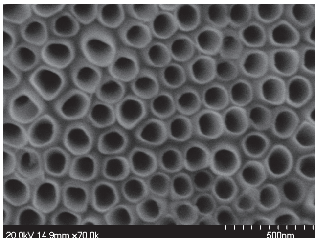
Figure 3 SEM top-view image of \text{TiO}_2 nanotubes after annealed at 450 °C.
