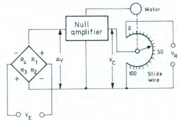
Figure Slide wire compensator principle
