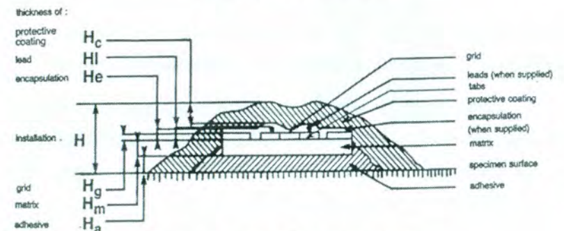
Figure b) Typical strain gauge installation Displacement of grid from specimen surface : H_d = H_s + H_m + 1/2 H_g
