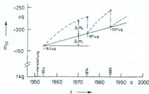
Fig. Changes in mass of the kilogram prototype No. 52. \Delta m_i irreversible, longstanding increase in mass. \Delta m_r reversible increase in mass due to surface layers that are removed by cleaning
