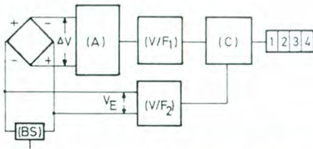
Figure Voltage to frequency conversion digitizing system
