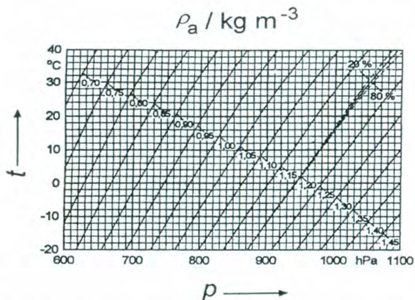
Fig. Roughly estimated determination of the air density \rho_a in \text{kg m}^{-3} at a relative air humidity h_r = 50\% , in the temperature range from -20^\circ\text{C} to +40^\circ\text{C} in the air pressure range from 600 hPa to 1100 hPa ( = \text{mbar} ).
