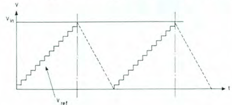
Figure Analogue/digital conversion with unit pulses
