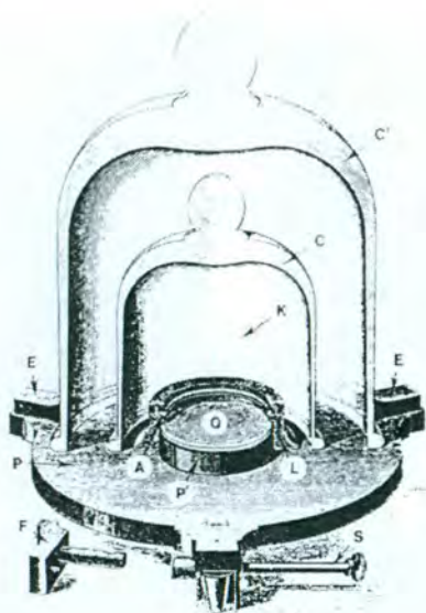
Fig. Sectional view of an original container for a kilogram prototype: K Pt-Ir kilogram prototype, Q Quartz plate as flat surface for the prototype, P, P Base plate (P) with brass cylinder (P'). A Brass crown (L) with silver ring (A) (inner diameter 42 mm) for protection against possible side movements of the prototype; C, C' Glass bell-jars secured against side movement by a ridge on the base plate (P), E, F Fixtures securing the outer glass bell-jar (C'). Fixture E is attached, Fixture F is removable, S Safety device for the removable fixture (F), The international prototype is additionally protected by a third glass bell-jar which lies on a polished glass plate (Fig. 22.6)
